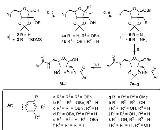
Scheme 1. Synthesis of compounds 8 f–I from 2 . Reagents and conditions (yields in parentheses): a) TBDMSCl, imidazole, DMF, 0°C, 16 h (63%); b) BnBr, NaH, DMF, 0°C, 16 h; c) TBAF, THF, RT, 4 h ( 4a 41.8%, 4b 42.5%); d) based on compound 4b : MsCl, Et 3 N, DCM, RT, 2 h (95%); e) NaN 3 , DMF, 90°C, 48 h (70%); f) PMe 3 , THF, H 2 O; g) ArCO 2 H, EDC·HCl, DMAP, HOBt, DMF, RT, 16 h; h) H 2 , Pd/C, HOAc, 5 h; i) 35% TFA, H 2 O, RT, 3 h. TBDMSCl = tert -butyldimethylsilyl chloride, DMF = N,N -dimethylformamide, Bn = benzyl, TBAF = tetra- n -butylammonium fluoride, THF = tetrahydrofuran, Ms = methanesulfonyl, EDC·HCl = 1-(3-dimethylaminopropyl)-3-ethylcarbodiimide hydrochloride, DMAP = 4-dimethylaminopyridine, HOBt = 1-hydroxybenzotriazole.
